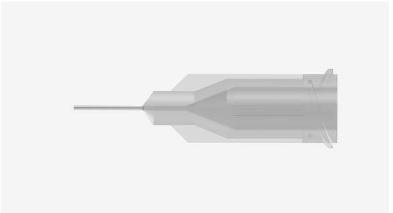
ND27S6 ØID 0.20 mm / 0.008 in
